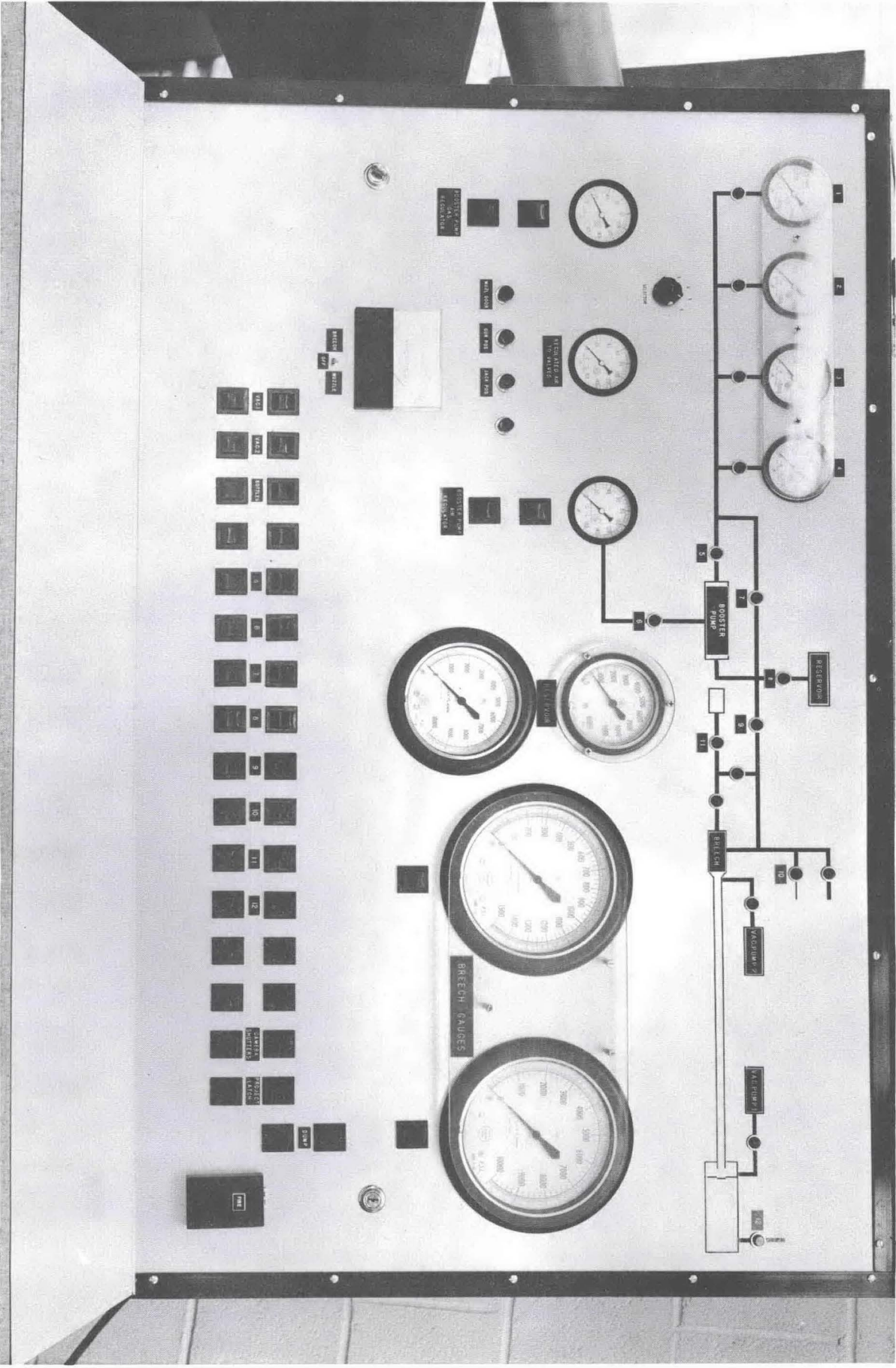
Fig. 14. Control panel.
